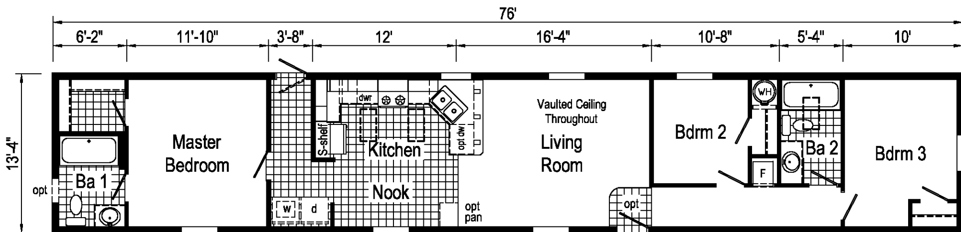
TS104-A 1476 Approx. 1013 Sq. Ft. S = Std. 4" staggered overhead cabinets
