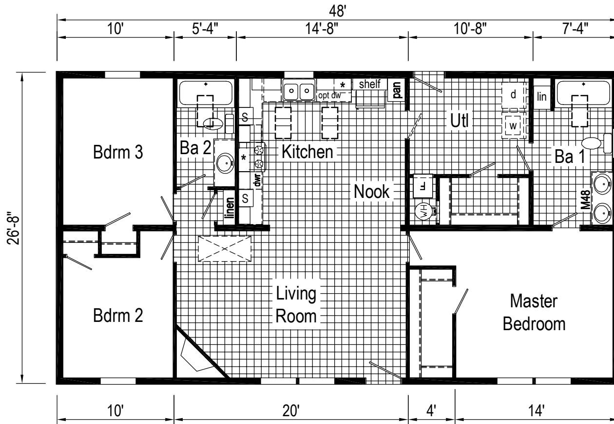
AH101-A6 2848 Approx. 1280 Sq. Ft.
