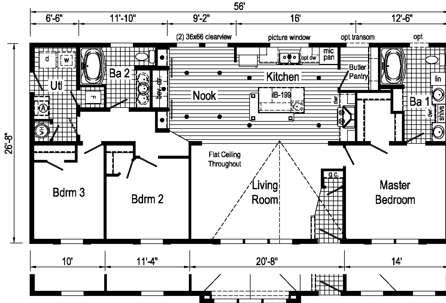
Opt. 26'-8" dormer w/ bump-out
