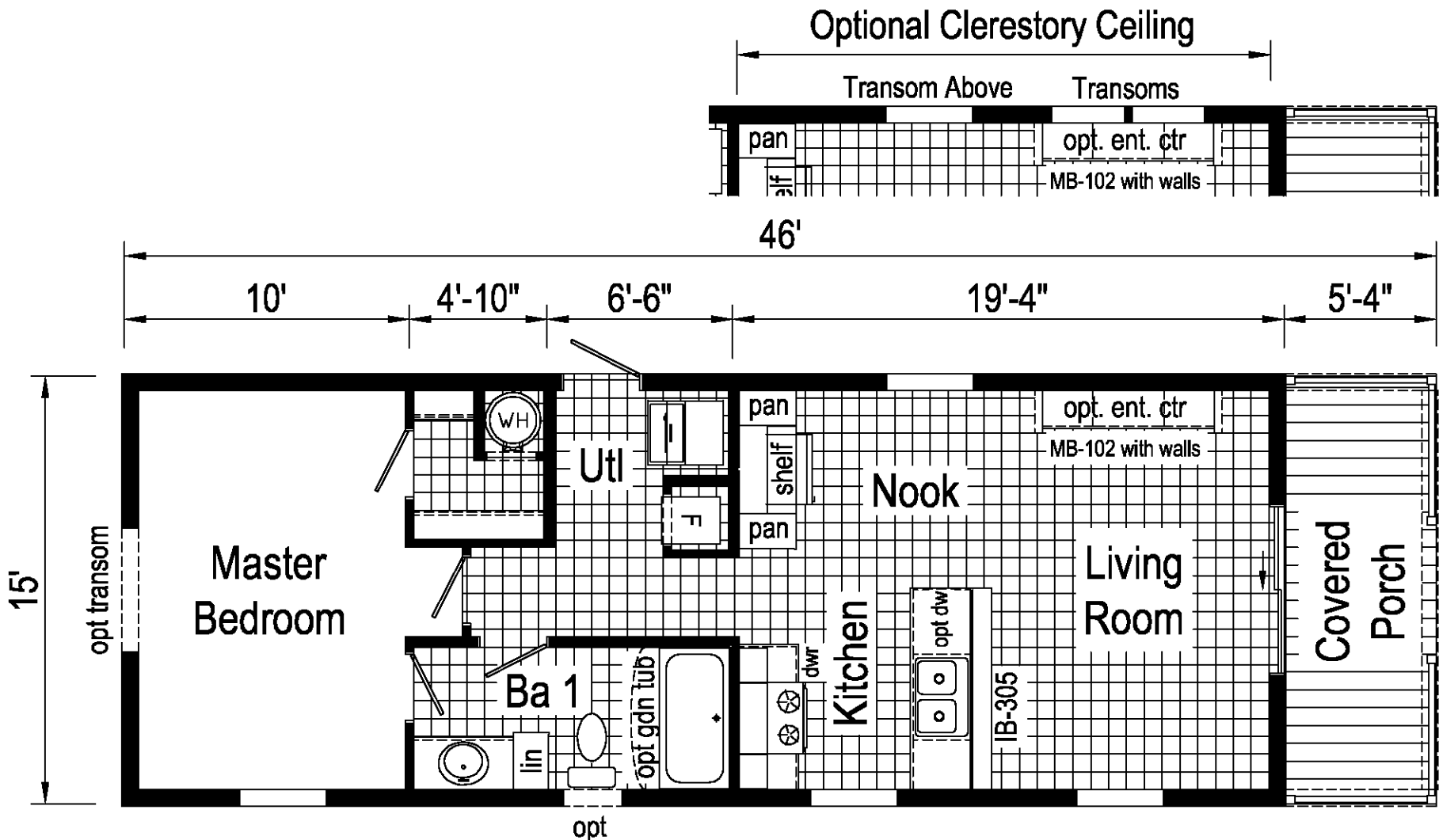
TT113-A 1646 Approx. 607 Sq. Ft.
