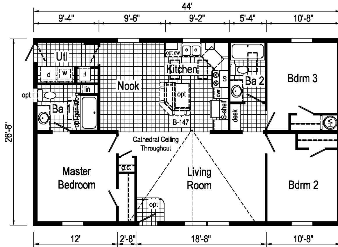
TD112-A 2844 Approx. 1173 Sq. Ft. S = Std. 4" staggered overhead cabinets
