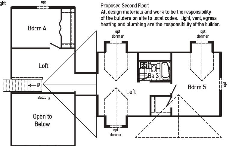
Proposed 2nd Floor with Optional 12/12 Chalet Roof
